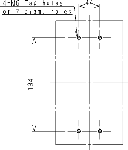
Drilling Plan
