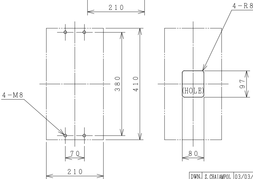
DRILLING PLAN.
