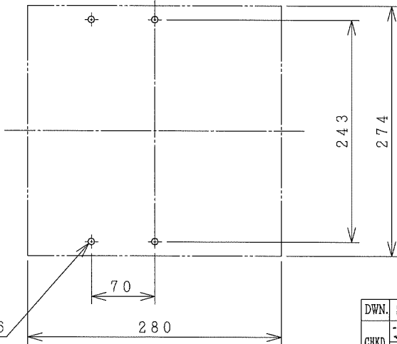
DRILLING PLAN.
