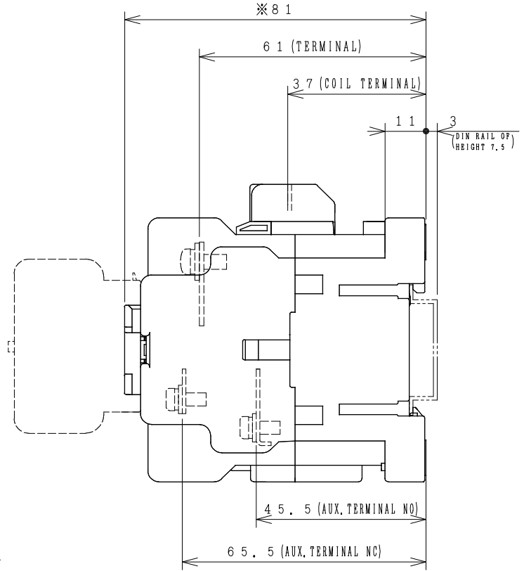
OUTLINE DIMENSIONS.
