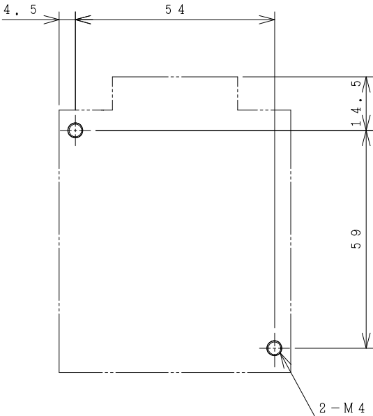
MOUNTING HOLES.
