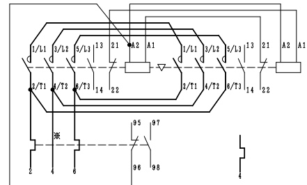
CONTACTS ARRANGEMENT.
