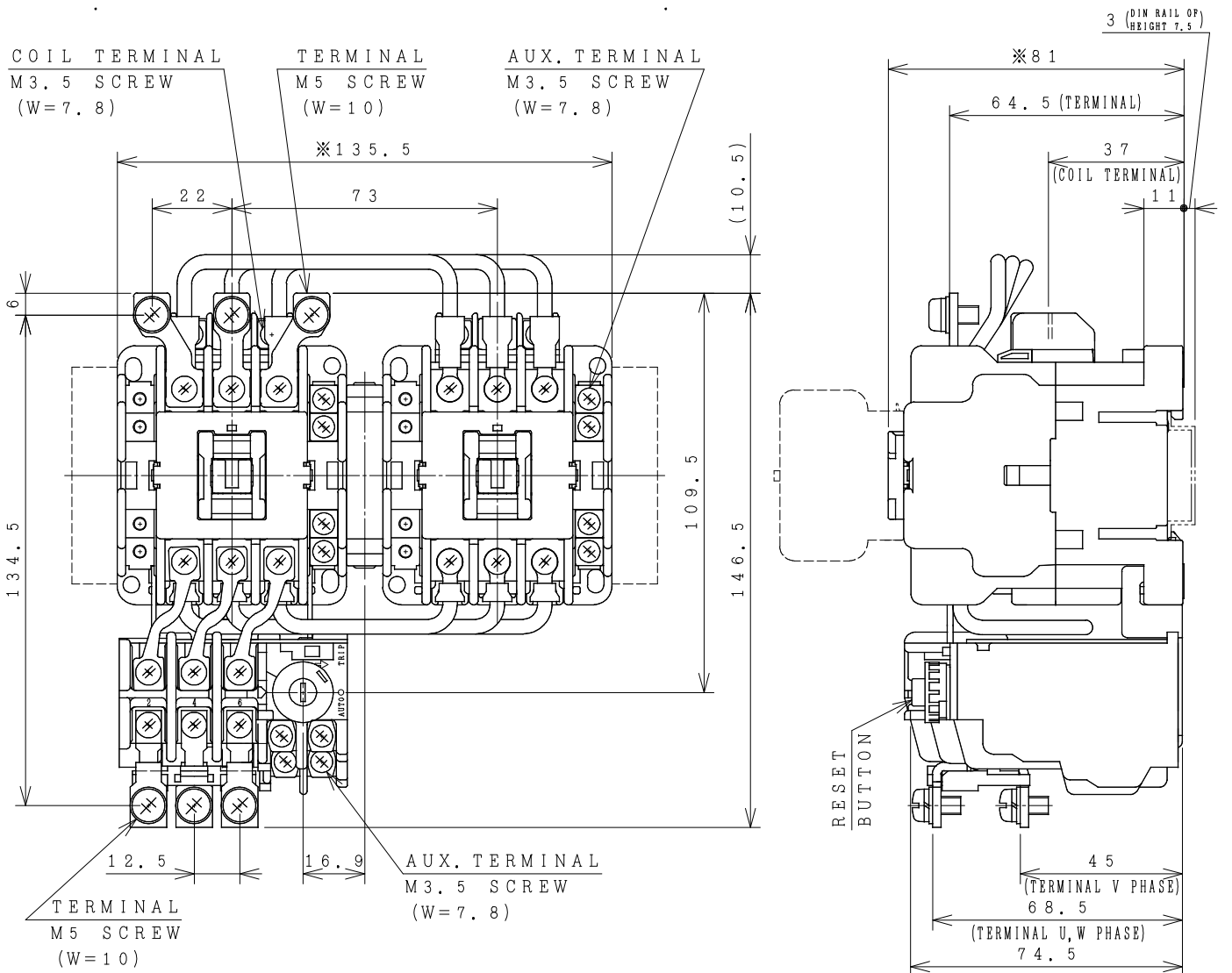
OUTLINE DIMENSIONS.
