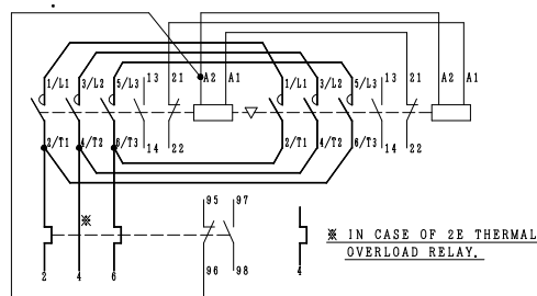
CONTACTS ARRANGEMENT.
