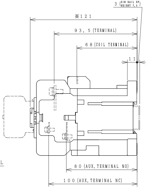
OUTLINE DIMENSIONS.
