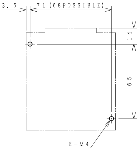
MOUNTING HOLES.
