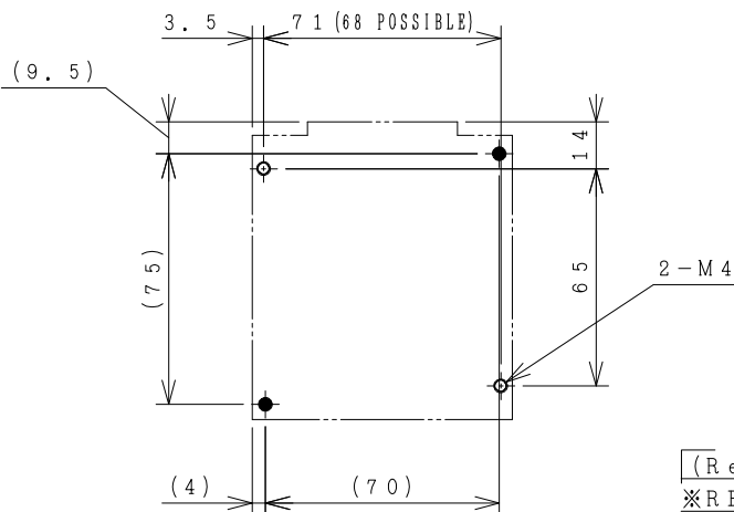
MOUNTING HOLES.
