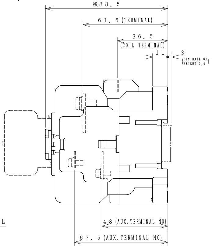
OUTLINE DIMENSIONS.
