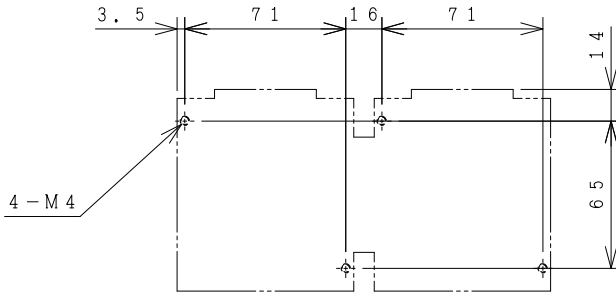
MOUNTING HOLES.
