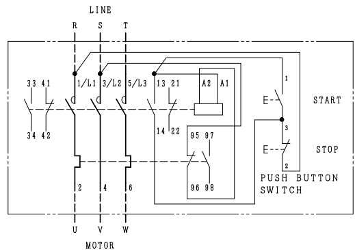
CONTACTS ARRANGEMENT.
