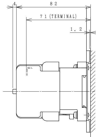
OUTLINE DIMENSIONS.
