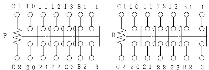
CONTACTS ARRANGEMENT.
