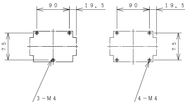
MOUNTING HOLES.
