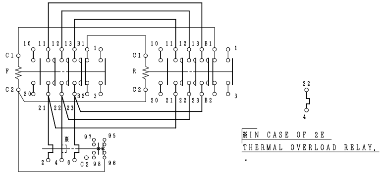
CONTACTS ARRANGEMENT.
