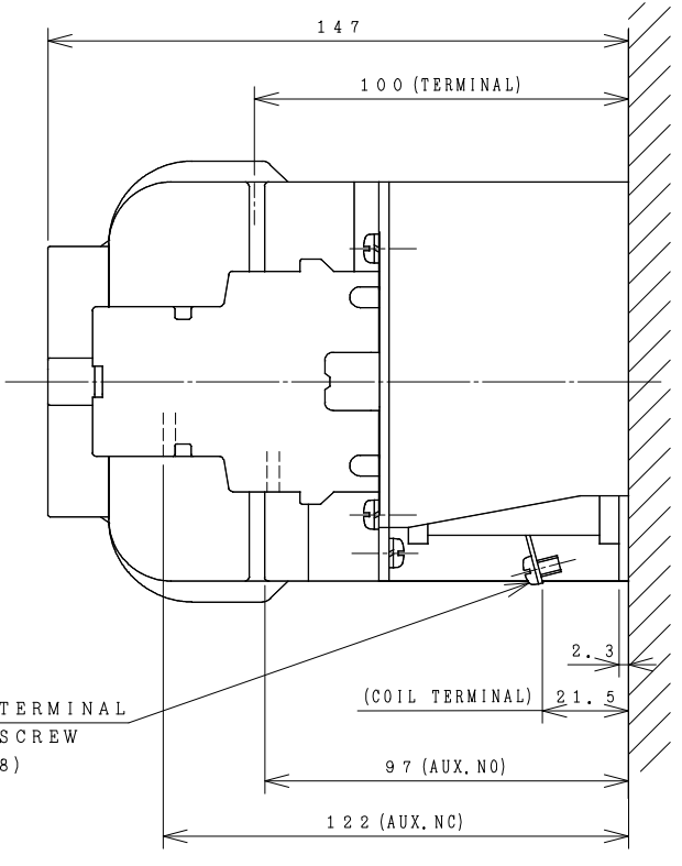
OUTLINE DIMENSIONS.
