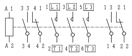
CONTACTS ARRANGEMENT.
