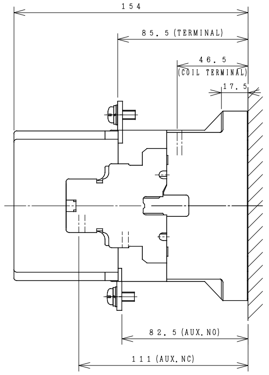
OUTLINE DIMENSIONS.
