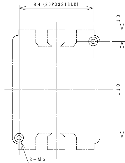
MOUNTING HOLES.
