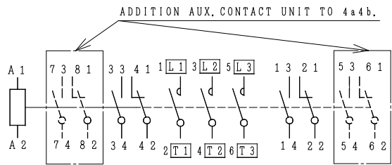
CONTACTS ARRANGEMENT.
