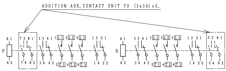
CONTACTS ARRANGEMENT.
