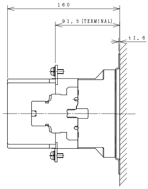
OUTLINE DIMENSIONS.
