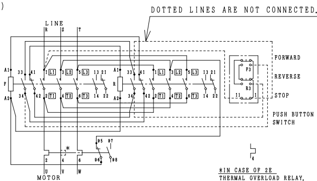
CONTACTS ARRANGEMENT.
