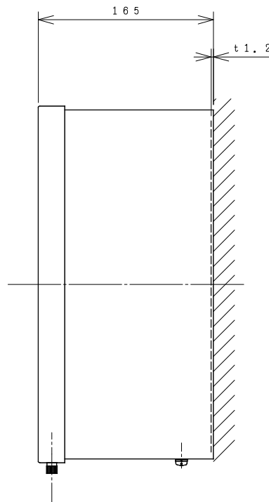
OUTLINE DIMENSIONS.
