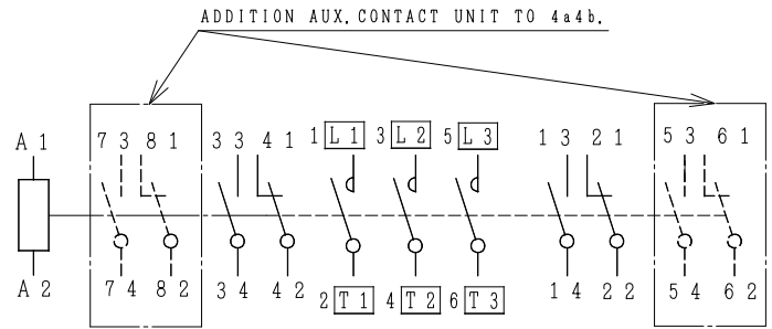
CONTACTS ARRANGEMENT.
