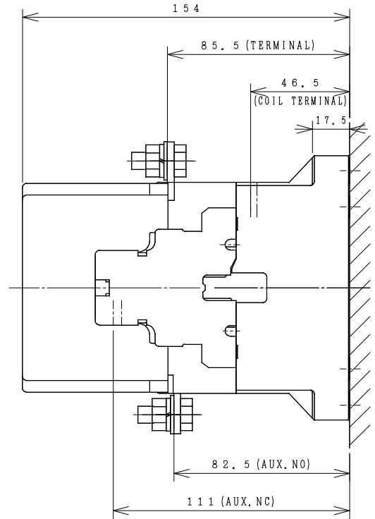
OUTLINE DIMENSIONS.
