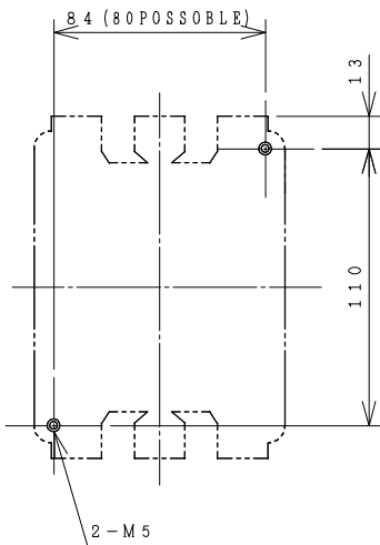
MOUNTING HOLES.
