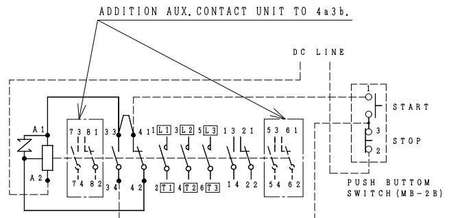
CONTACTS ARRANGEMENT.
