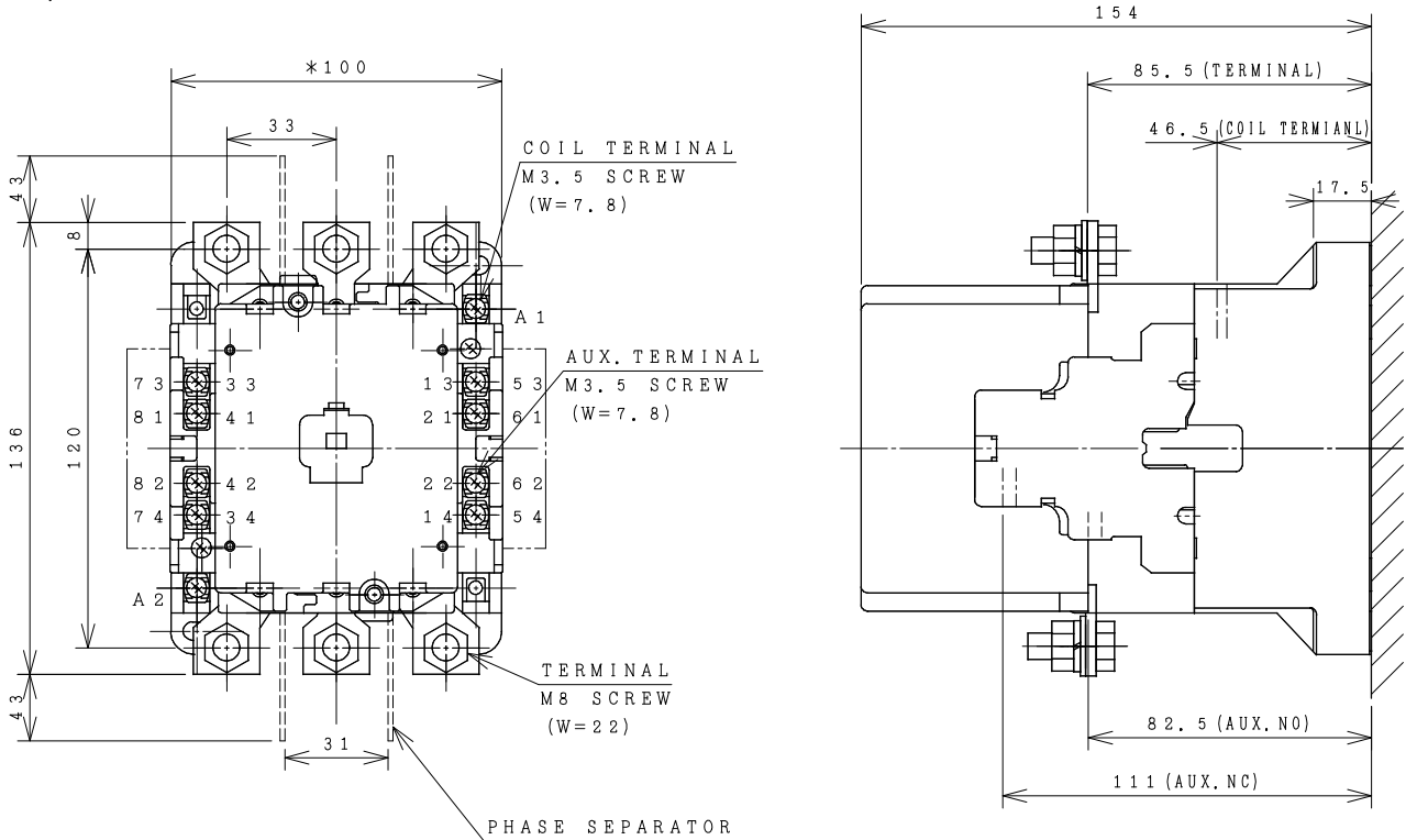
OUTLINE DIMENSIONS.
