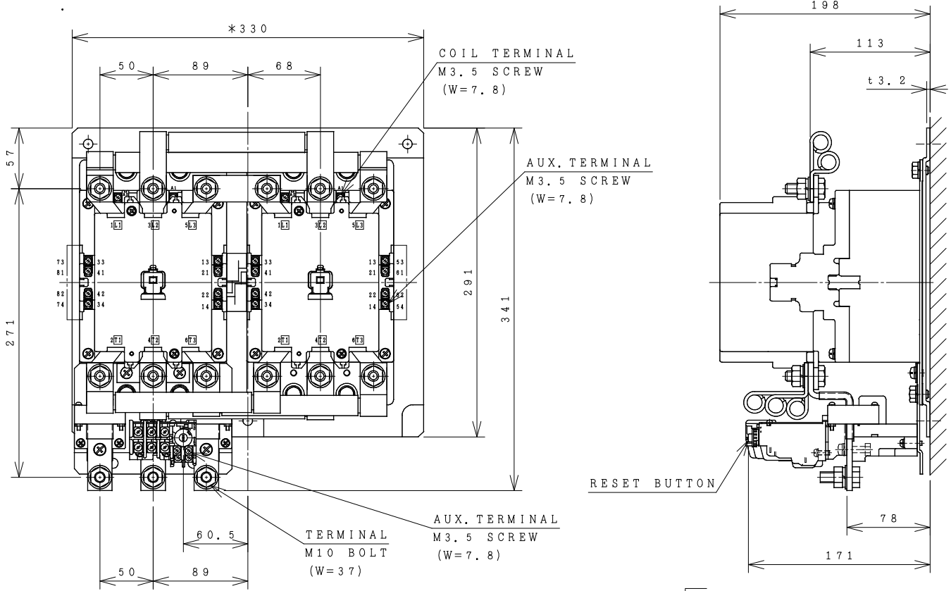
OUTLINE DIMENSIONS.
