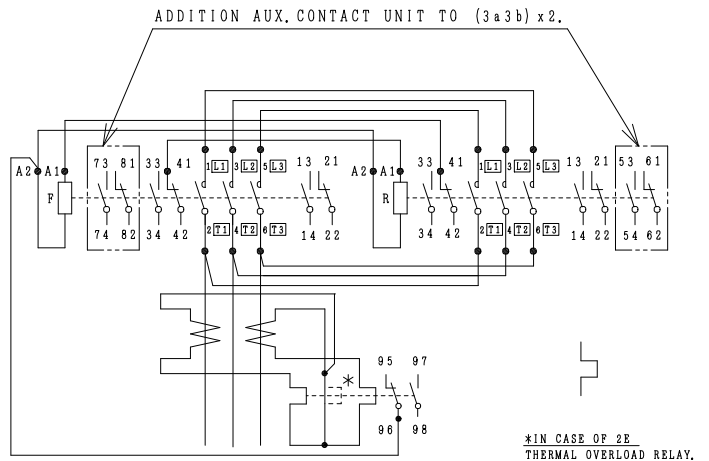
CONTACTS ARRANGEMENT.
