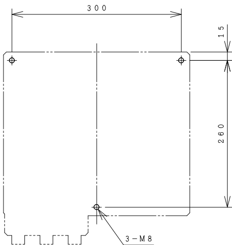
MOUNTING HOLES.
