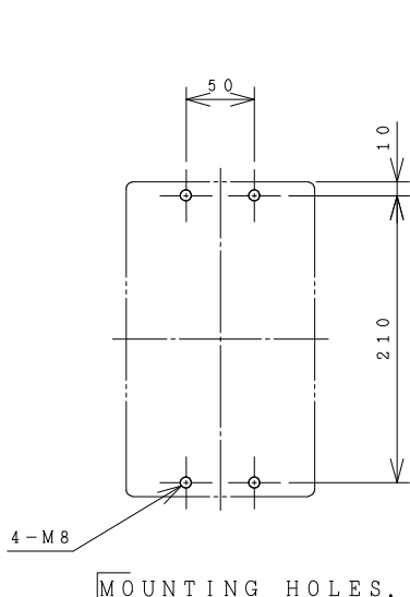
MOUNTING HOLES.
