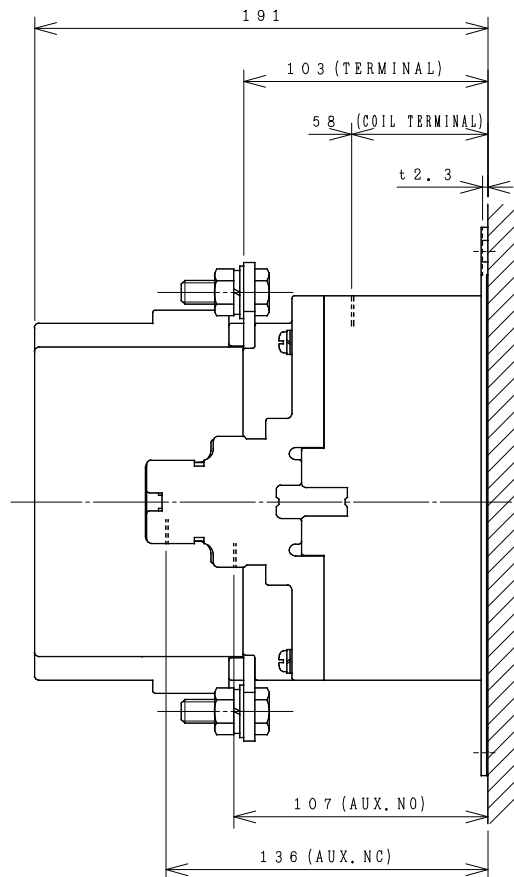
OUTLINE DIMENSIONS.
