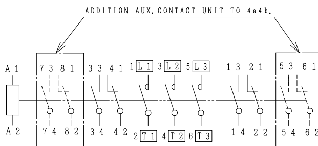
CONTACTS ARRANGEMENT.
