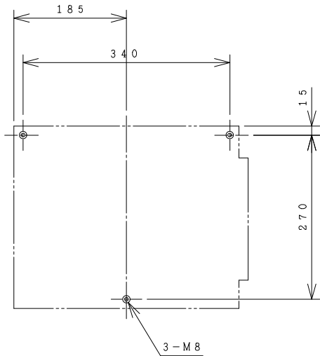
MOUNTING HOLES.
