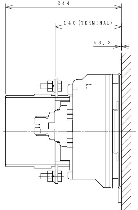
OUTLINE DIMENSIONS.
