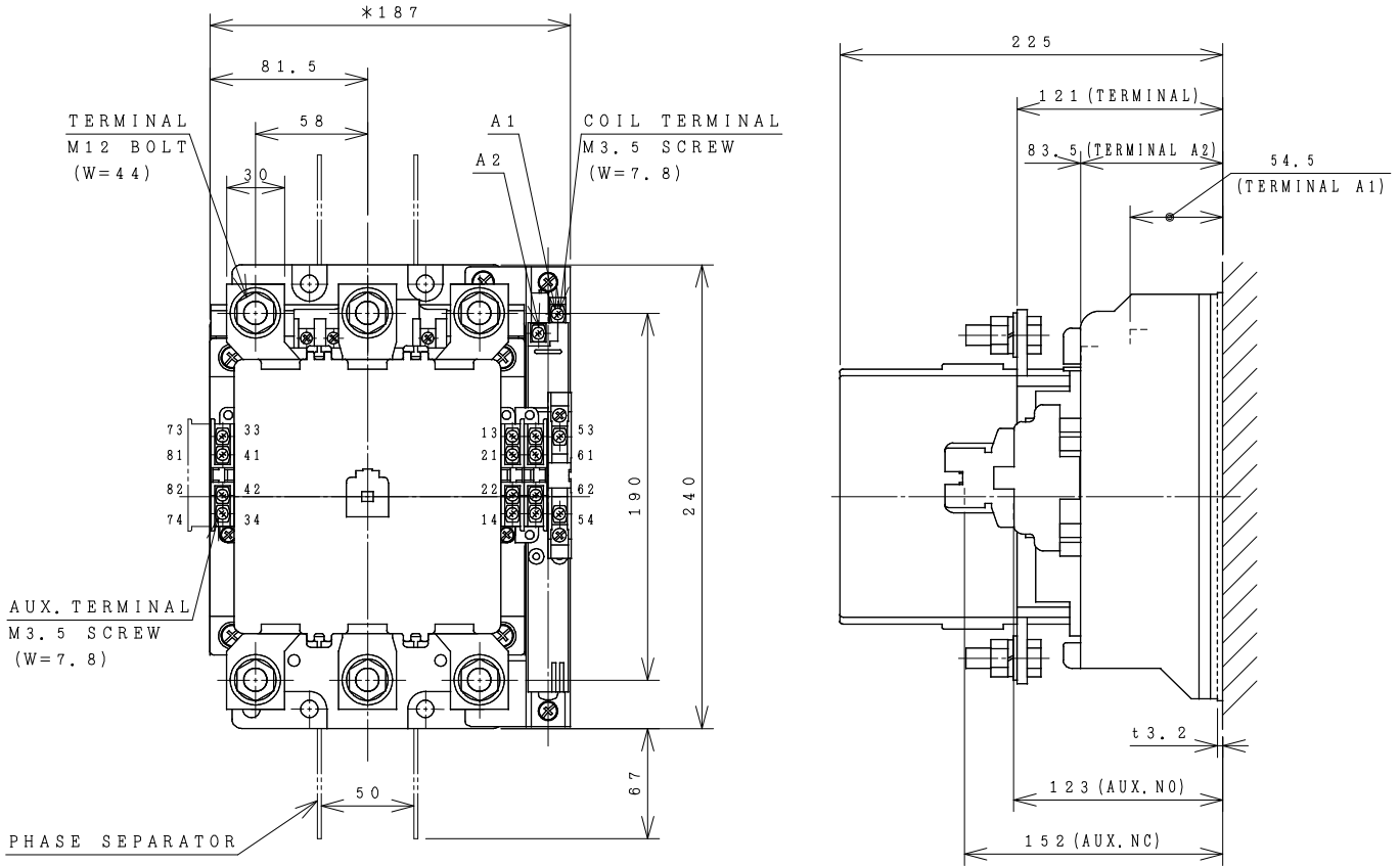
OUTLINE DIMENSIONS.
