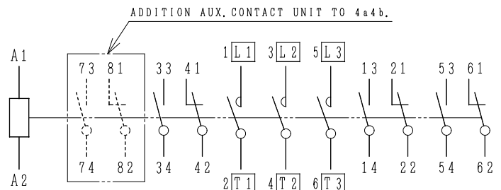
CONTACTS ARRANGEMENT.
