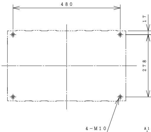
MOUNTING HOLES.
