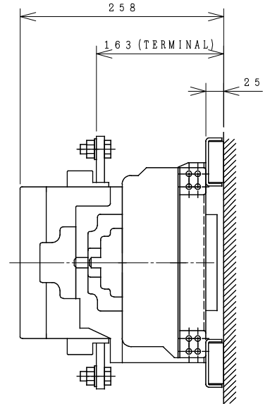
OUTLINE DIMENSIONS.
