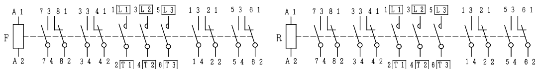
CONTACTS ARRANGEMENT.
