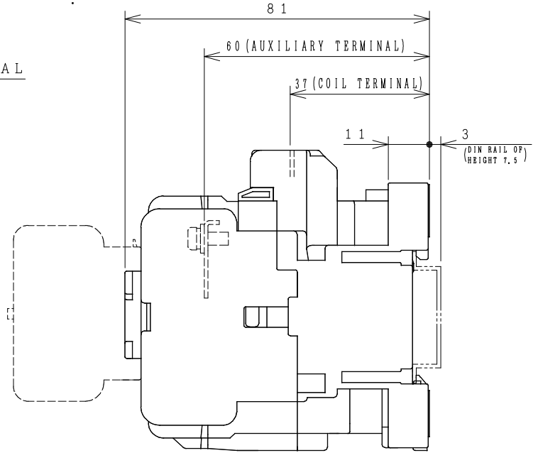
OUTLINE DIMENSIONS.
