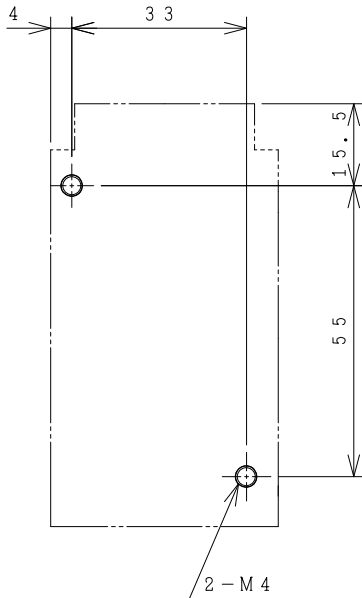
MOUNTING HOLES.
