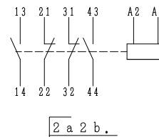
CONTACTS ARRANGEMENT.
