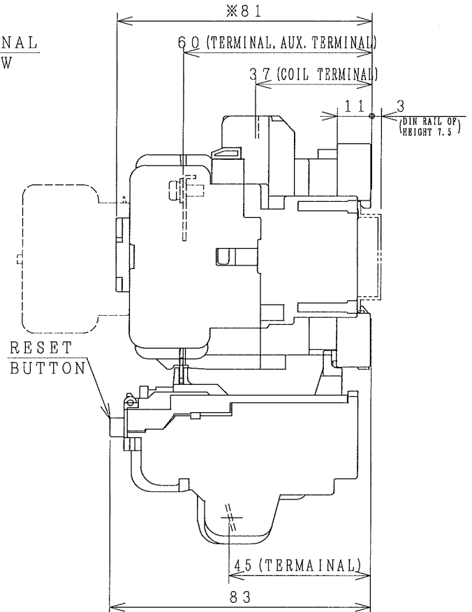
OUTLINE DIMENSIONS.
