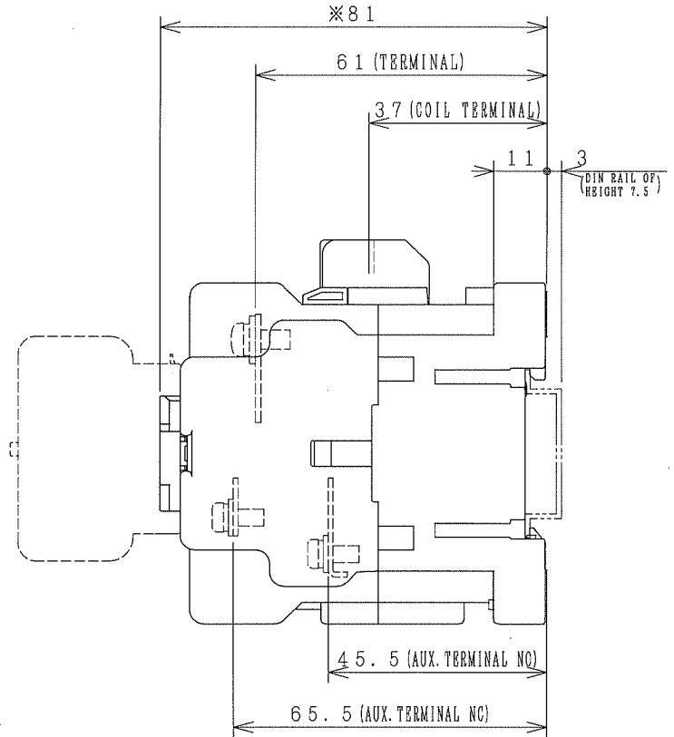
OUTLINE DIMENSIONS.
