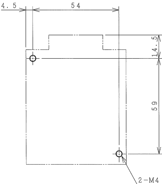
MOUNTING HOLES.
